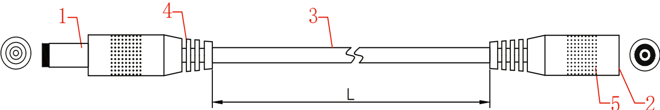
WIRING DIAGRAM
