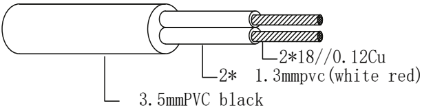
24AWG 2C POWER CORD
