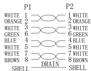
WIRING DIAGRAM
