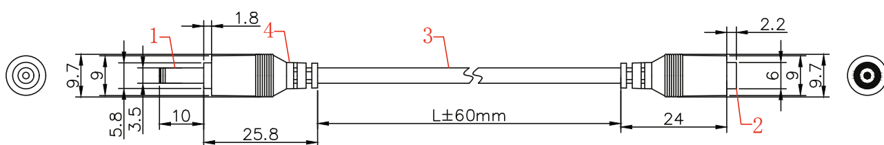
WIRING DIAGRAM
