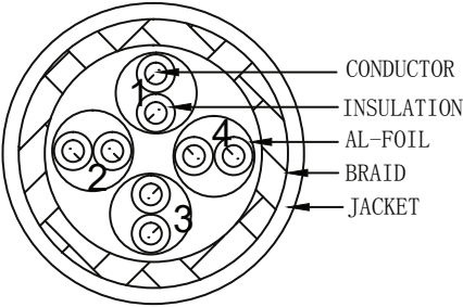
PIN OUT
